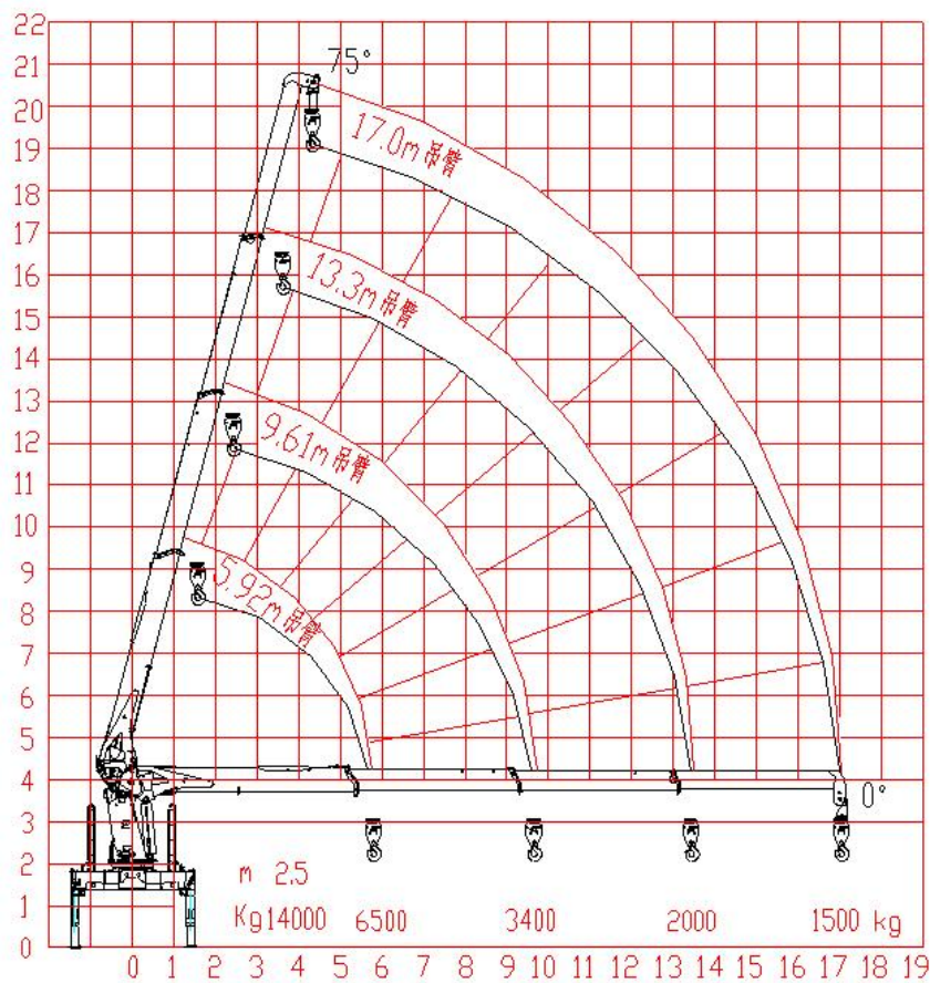
Lifting chart
